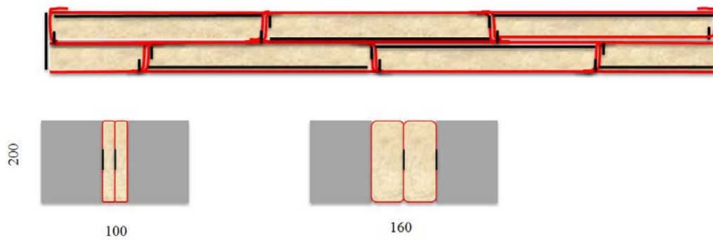
Figure 4 Top view and cross sections of semi-brick bond lay-out applied Firetight®
