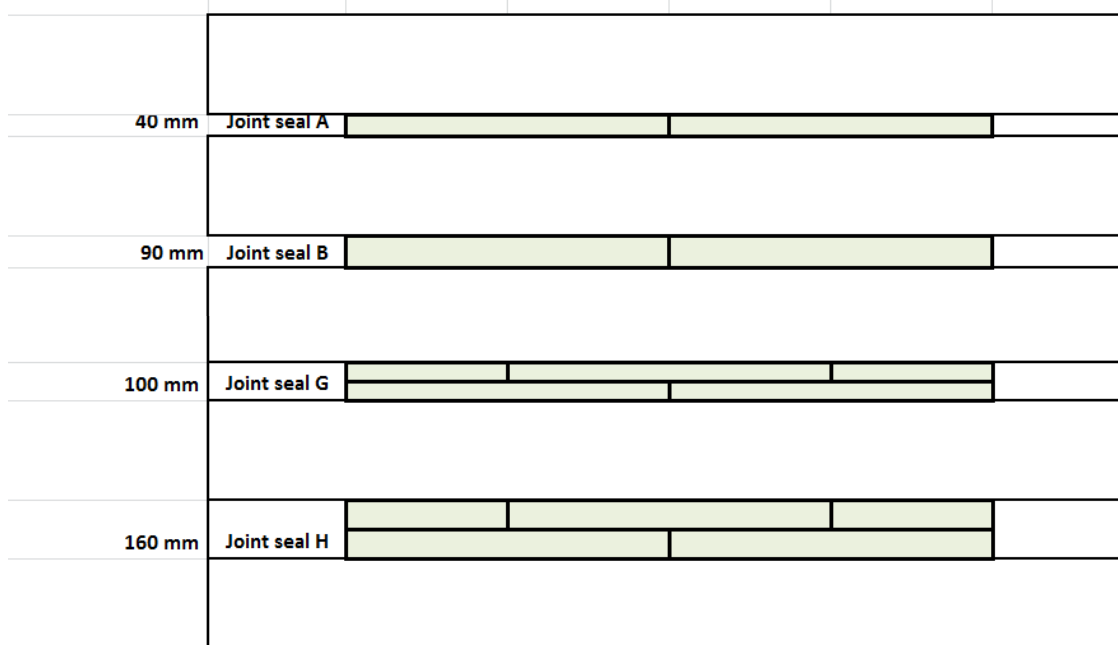
Figure 1 Lay-out of Alert Firetight® test
